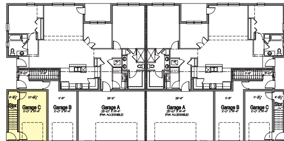
1st Floor Building Plan - 6 Unit
