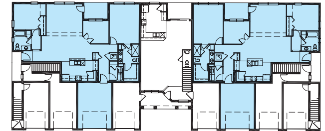
BUILDING 1ST FLOOR
